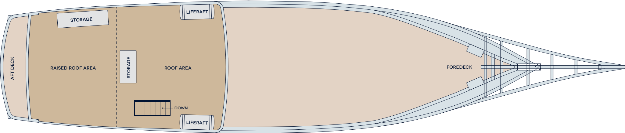
ROOF DECK
